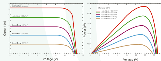
Current-Voltage & Power-Voltage Curves(SP470M-48H)
