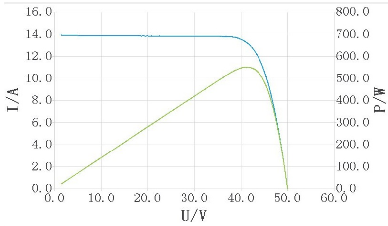
Fig. 5 IV curve of module No.1 Serial number: SE00157222030400121
