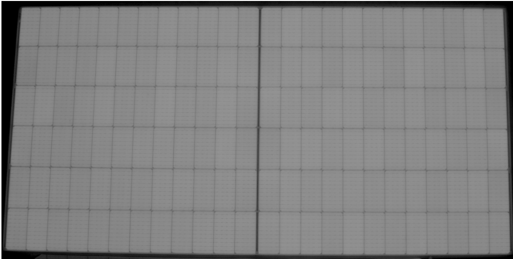
Fig. 6 EL photo of module No.1 Serial number: SE00157222030400121
