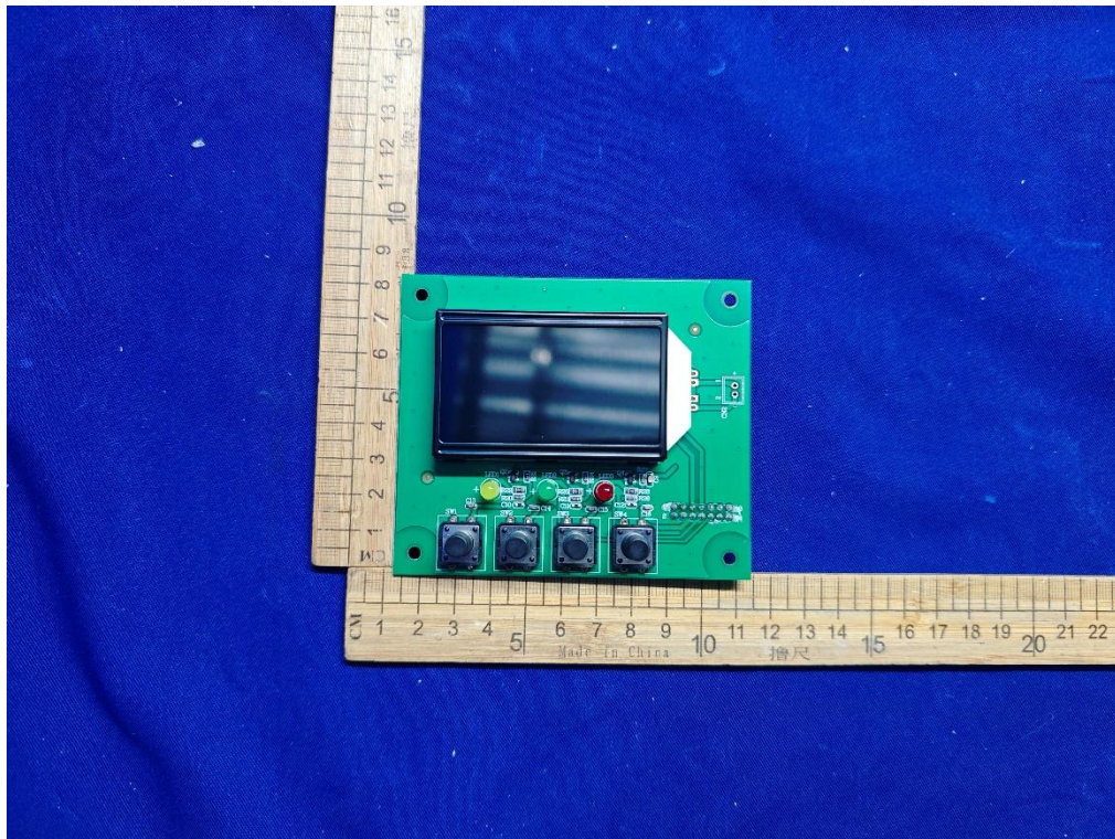
Fig. 15 -- PCB view
