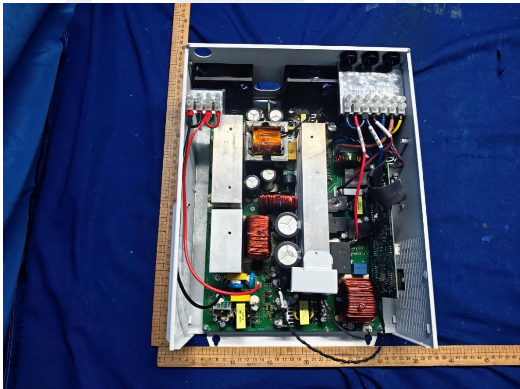
Fig. 6 -- Internal view 1
