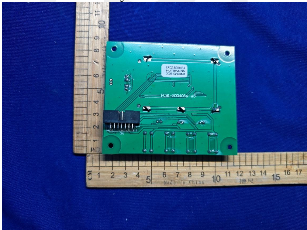
Fig. 16 -- PCB view
